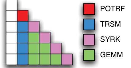
Figure 3. Step k of a Cholesky factorization.
