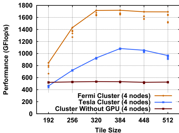
Figure 6. Performance of the Cholesky factorization as a function of the tile size, for a problem size of 34560 (Dancer cluster, 4 nodes).
