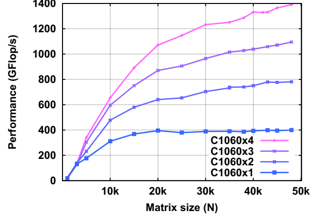
Figure 5. Multiple Teslas (C1060) Performance of Cholesky factorization according to problem size (Mordor, single node).
