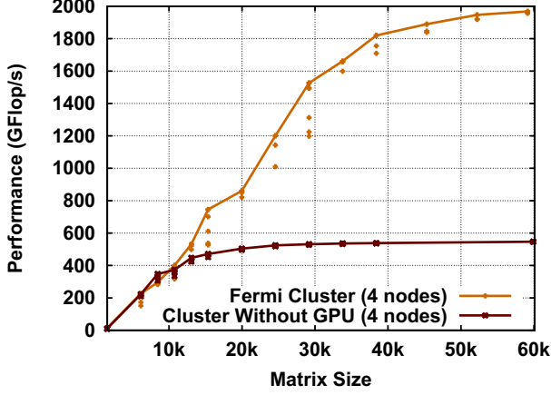
Figure 8. Problem Scaling: performance of the Cholesky factorization as a function of the problem size, (4-node Fermi Cluster).
