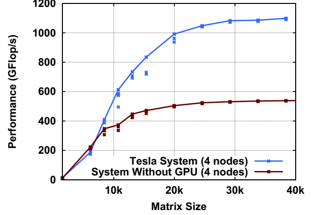
Figure 9. Problem Scaling: performance of the Cholesky factorization as a function of the problem size, (4-node Tesla Cluster).
