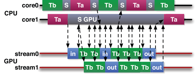
Figure 1. Schematic (not to scale) DAGuE execution, on a GPU enabled system; kernels Ta and Tb alternate with scheduling actions (S) and in/out GPU asynchronous memory accesses.
