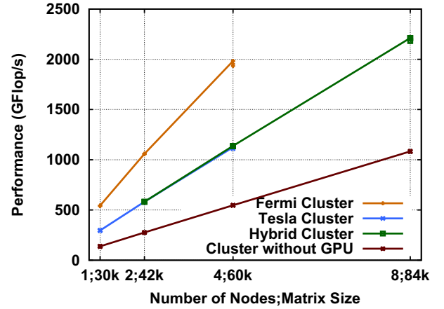
Figure 7. Weak Scalability: performance of the Cholesky factorization as a function of the number of nodes, with a problem size scaled accordingly (Dancer cluster).
