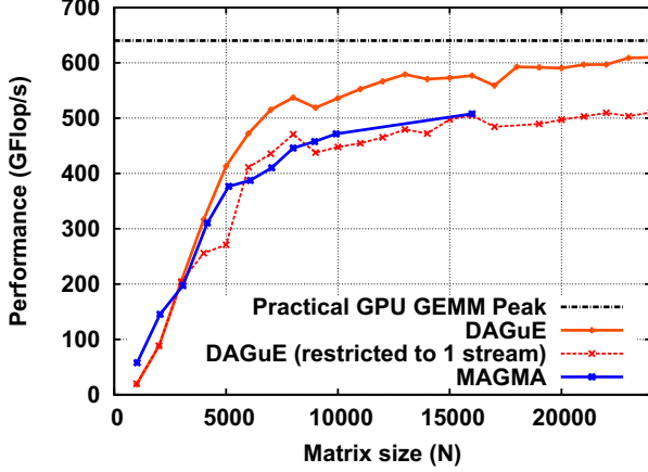
Figure 4. Fermi (C2050) Performance of Cholesky factorization according to problem size. Comparison between DAGuE and MAGMA (Dancer, single node).
